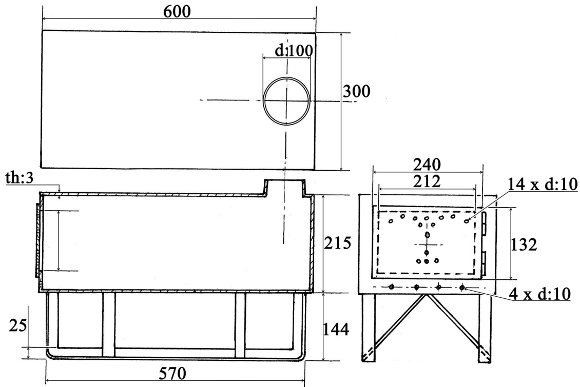
STOVE/HEATER, wood/coal, rectangular, horizontal, for tent
